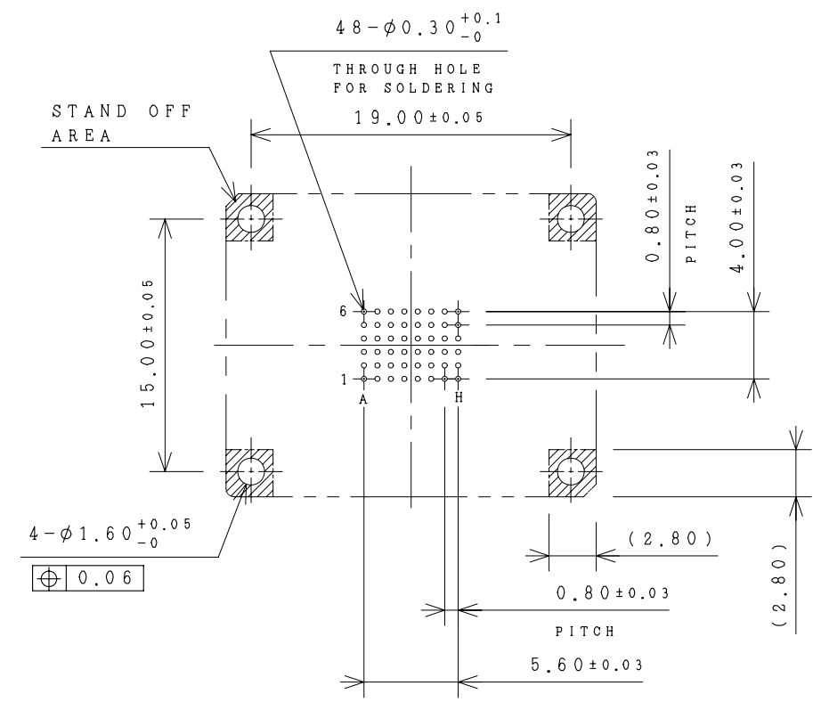
P. C. B. HOLE PATTERN (TOP VIEW)
